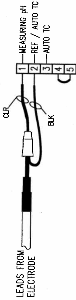
pH ELECTRODE WITH NO TEMP. COMP.
